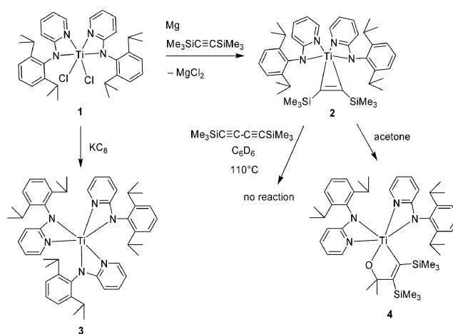
Scheme 1. Synthesis of 2 , 3 , and 4 .
