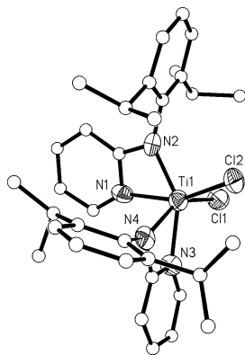
Figure 1. Molecular structure of 1 (ellipsoids correspond to the 50% probability level). Hydrogen atoms and two toluene molecules are omitted for clarity; selected bond lengths (Å) and angles (°): N1–Ti1 2.179(8), N2–Ti1 1.954(6), N3–Ti1 2.124(7), N4–Ti1 2.036(7), C11–Ti1 2.310(3), C12–Ti1 2.247(3); N4–Ti1–N3 63.2(3), N2–Ti1–N1 63.8(3), C12–Ti1–C11 93.76(10).
