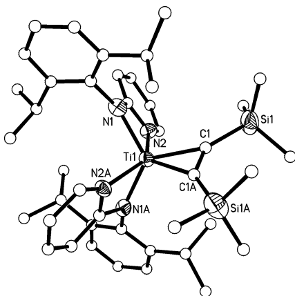
Figure 2. Molecular structure of 2 (ellipsoids correspond to the 50% probability level). Selected bond lengths (Å) and angles (°): C1–C1A 1.338(13), C1–Ti1 2.090(7), Ti1–N1 2.058(5), Ti1–N2 2.152(5); C1–C1A–Si1 138.9(2), C1–C1A–Ti1 71.33(18), N1–Ti1–N1A 121.4(3), C1–Ti1–C1A 37.3(4), N1–Ti1–N2 64.22(18).
